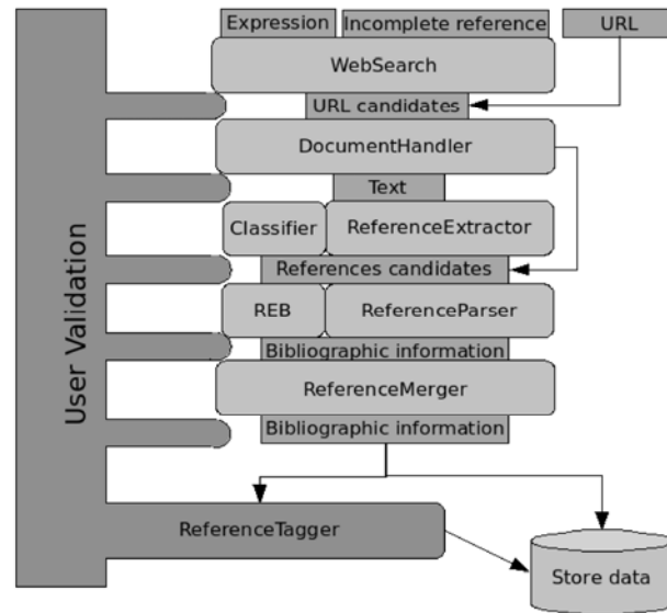
Figure 1. SUPeRB architecture
